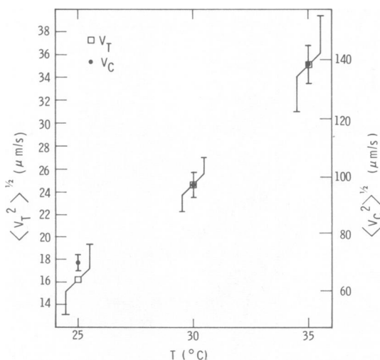
FIGURE 2 Temperature dependence of \langle V_T^2 \rangle^{1/2} and \langle V_C^2 \rangle^{1/2} . The error bars represent our estimate of confidence limits based on the repeatability of measurements at each temperature.
