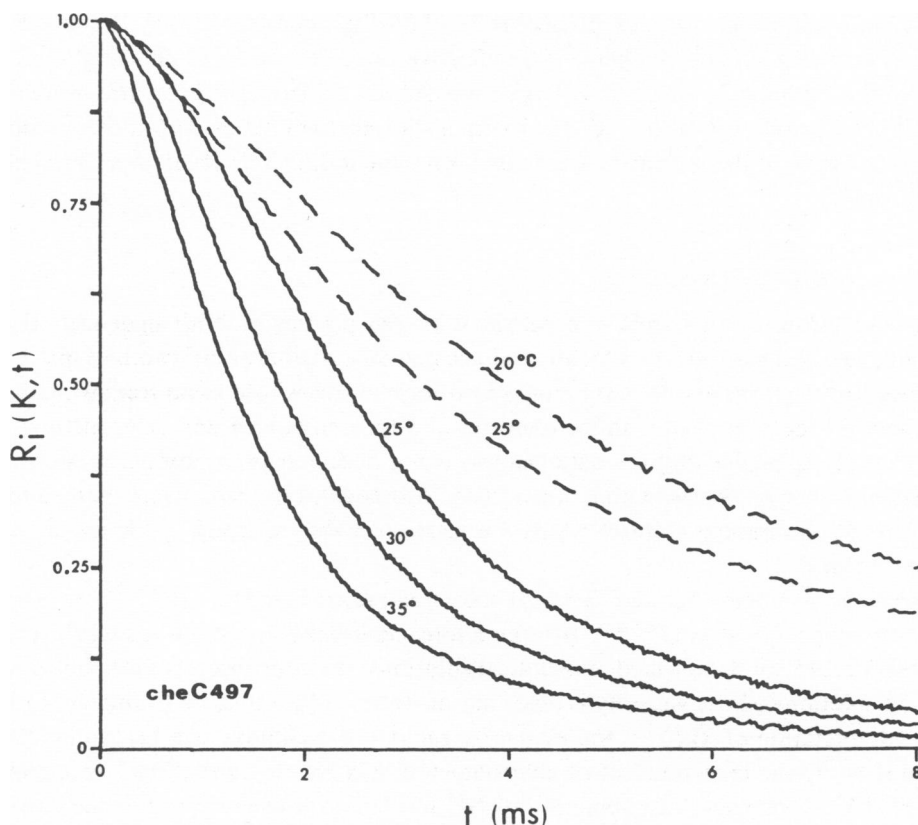
FIGURE 3 Photocurrent correlation function at high population densities (interference fluctuations) for bacteria grown at 25°C (broken lines) and 30°C (solid lines). Measurement temperatures are indicated above the curves.
