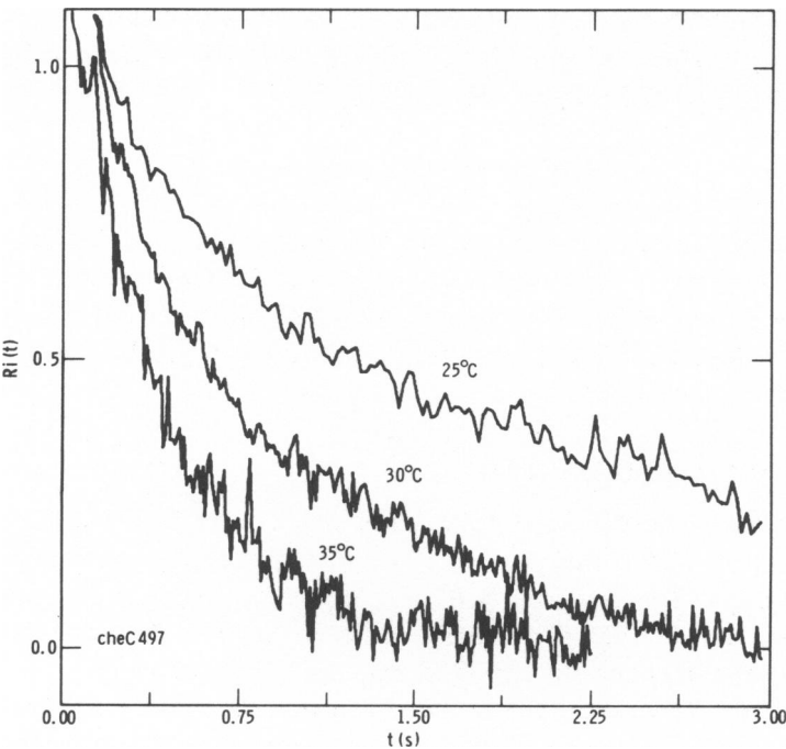
FIGURE 1 Photocurrent correlation function at low population densities (number fluctuations).
